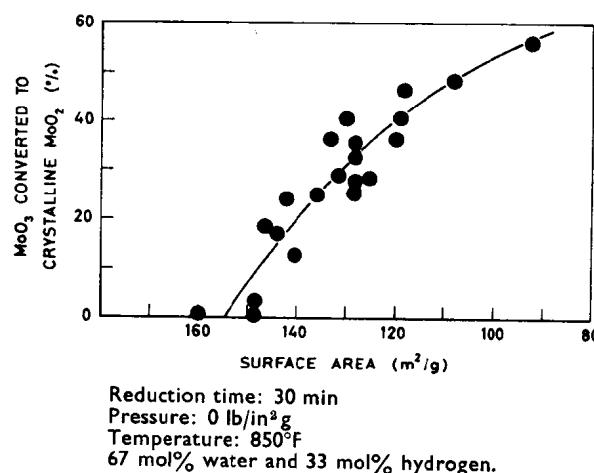
Fig. 6.—The effect of surface area on the formation of crystalline molybdena ( \text{MoO}_2 )
