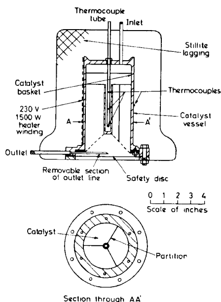
Fig. 5.—Catalyst stability—catalyst vessel assembly of test unit
