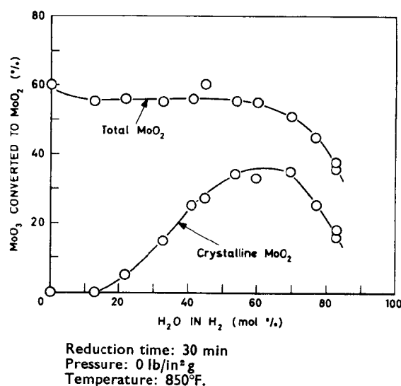
Fig. 5.—The effect of water partial pressure on the formation of crystalline molybdena ( \text{MoO}_2 )
