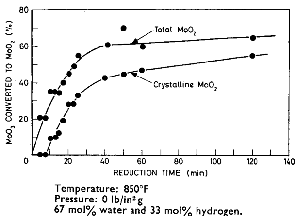
Fig. 3.—The effect of reduction time on the formation of crystalline molybdena ( \text{MoO}_2 )
