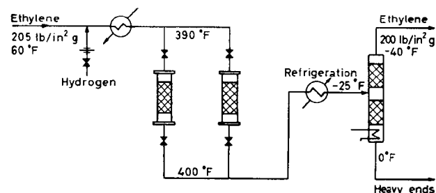
Fig. 2.—Acetylene hydrogenation unit
