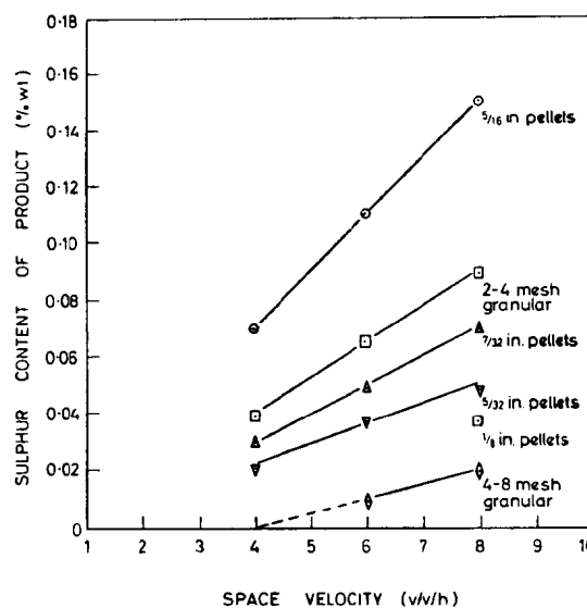
Fig. 9.—Effect of particle size on hydrofining activity of cobalt/molybdenum catalysts
