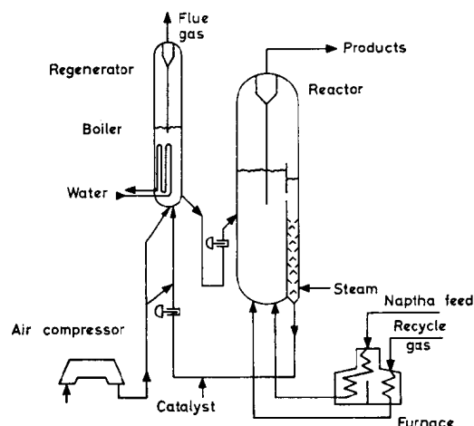
Fig. 1.—Fluidised-bed hydroformer
