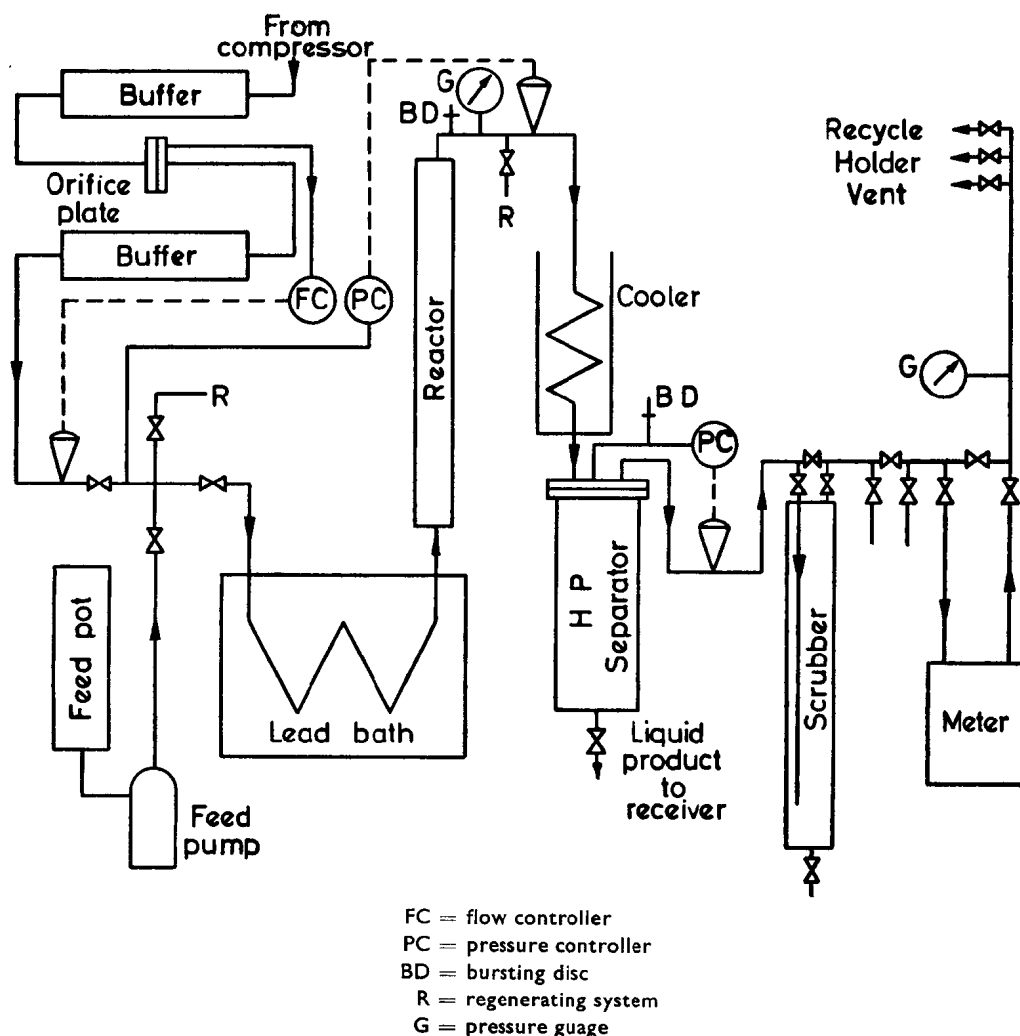
Fig. 1.—Pilot plant for catalytic desulphurisation
