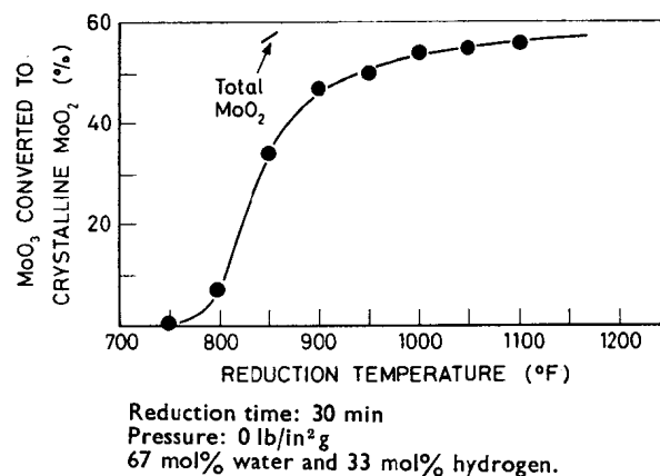
Fig. 4.—The effect of temperature on the formation of crystalline molybdena ( \text{MoO}_2 )
