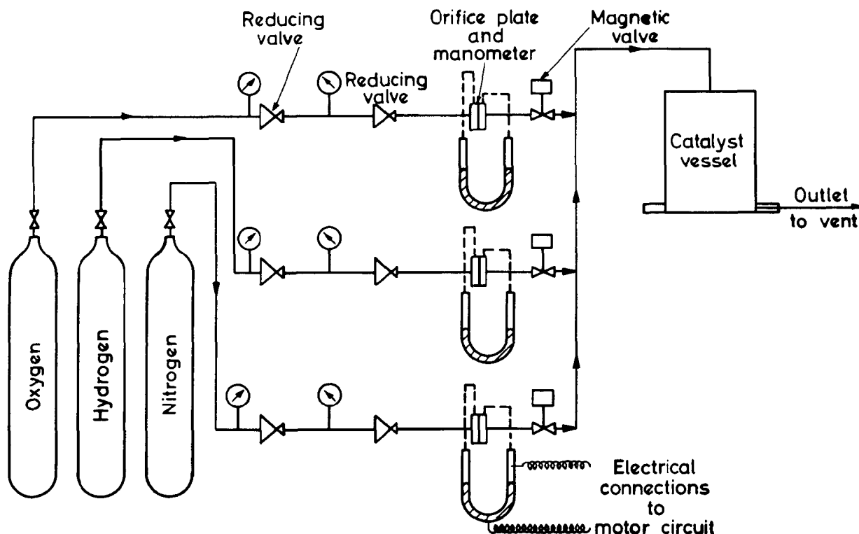
Fig. 4.—Catalyst stability—flow diagram of test unit
