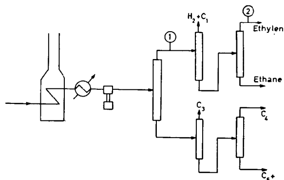
Fig. 1.—Possible locations for acetylene hydrogenation in an ethylene plant
