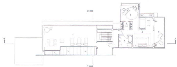
Third floor layout plan
