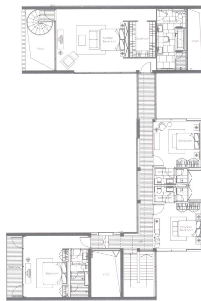
Second floor layout plan
