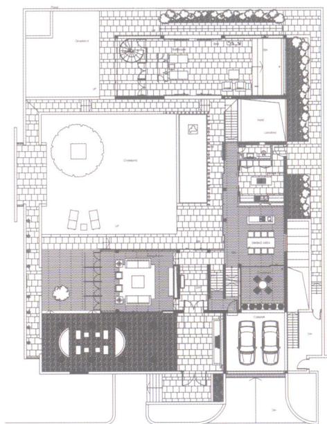
Ground floor layout plan
