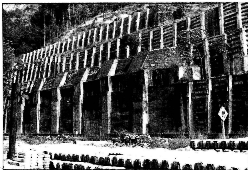
插旗山锚杆挡墙
