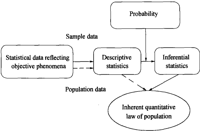
Figure 1. 2 Relationship between descriptive and inferential statistics
