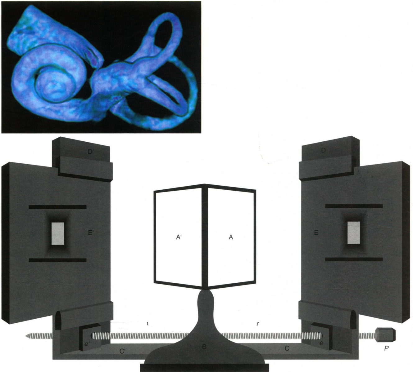
Fig. 1.1 Reconstructed 3D cochlea and reflecting mirror stereoscope
