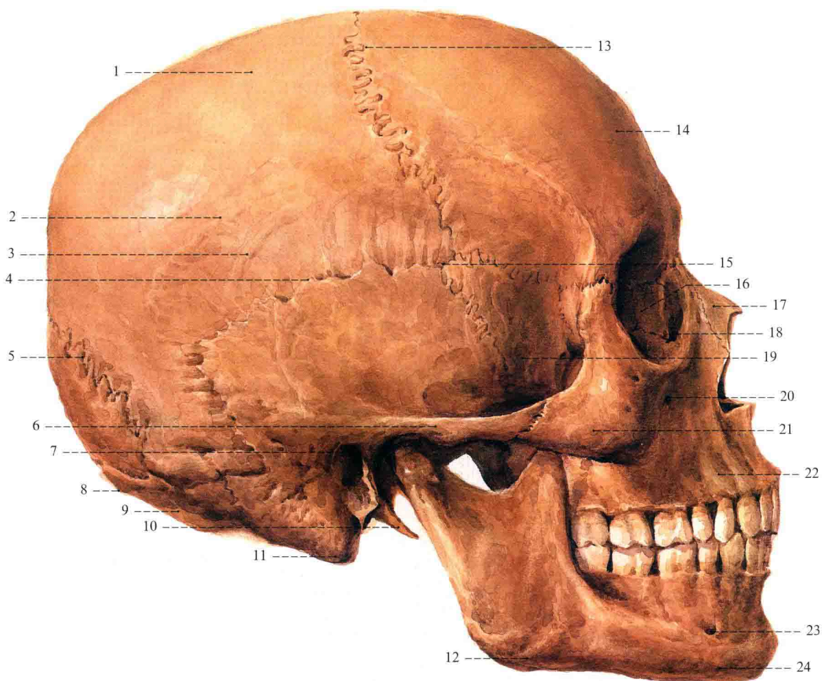
2. 颅 (侧面观)
