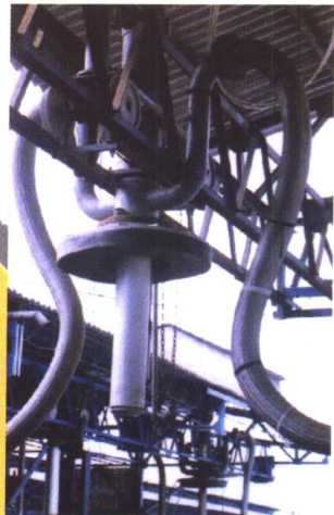
汽柴油密闭装车装置 sealed loading device for gasoline with ration
