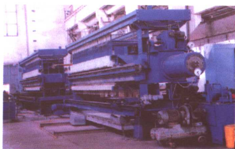
全自动厢式压滤机 series of chamber full-automatic pressure filter 1~500m 2
