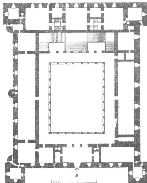
ALCAZAR OF TOLEDO.
