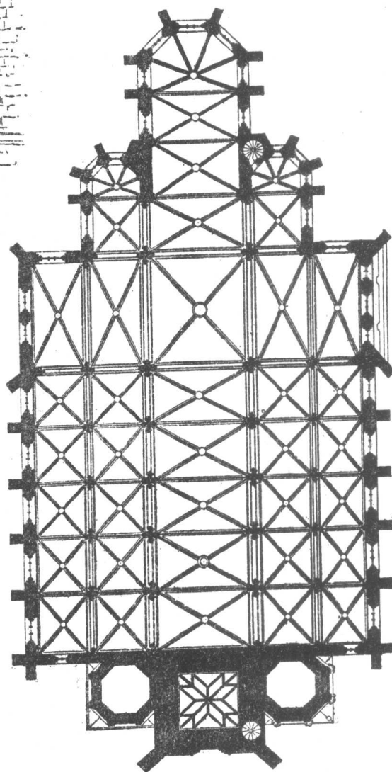
AISLED: A FIVE-AISLED CHURCH; CHURCH OF S. MARY, MULHAUSEN, PRUSSIA, GERMANY.
