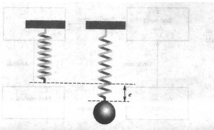
Figure 1.2 Spring-mass system
