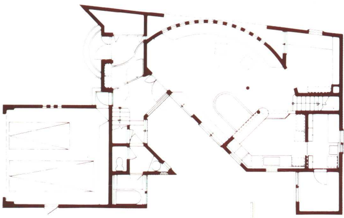
一楼 (123.60m 2 )
