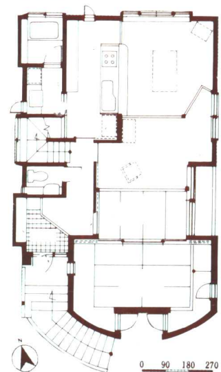
一楼 (78.15m²)
