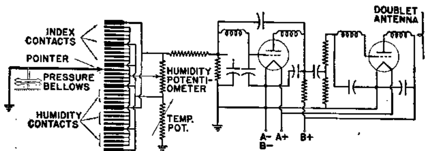
Basic circuit of a typical radiometeorograph.
