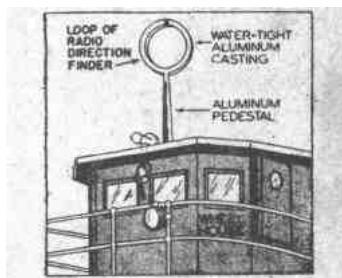
Radio direction-finder loop installation above the wheelhouse of a vessel, and loop characteristics.
