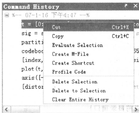
图 1-6 Command History
