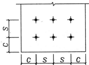
图4.4 锚栓间距及边距
