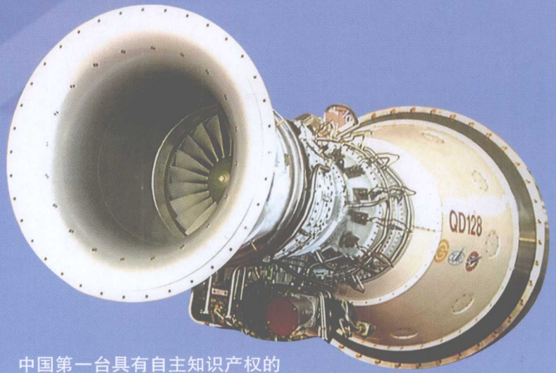
中国第一台具有自主知识产权的 QD-128 燃气轮机在黎明公司诞生 The Birthplace of QD-128 Gas Turbine (The First One in China Provided with Independent Intellectual Property)
