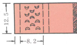
(6)鱼身外套展开图。用刀 刻出鱼鳞;
