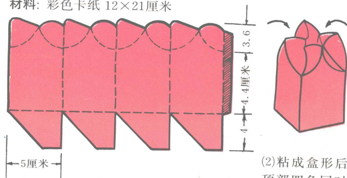
(1)花形盒展开图;
