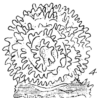
2-4 Cratiomyxa fruticulosa
