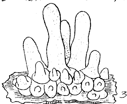
2-4 Cratiomyxa fruticulosa
