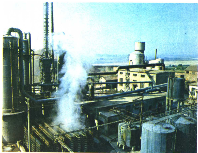
磷肥厂沸腾炉
