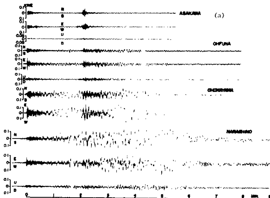
Fig.2 Seismograms obtained by array observation during the foreshocks of the Near Izu-Ohshima Earthquake of Jan.14,1978(09:45 and 09:47,M=4.9, D=0km)(a) and the Off Miyagi Earthquake of Feb.20,1978(M=6.7,D=50km)(b).
