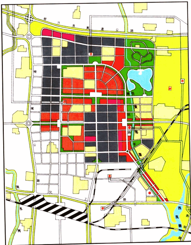
郑州高新技术产业开发区规划总图 The planning map of Zhengzhou High & New Technology Industries Development Zone.
