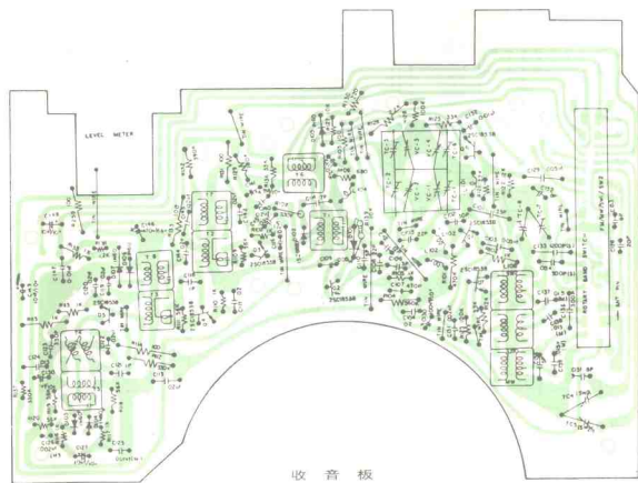
4. CARISON 858S型收录机印刷电路板
