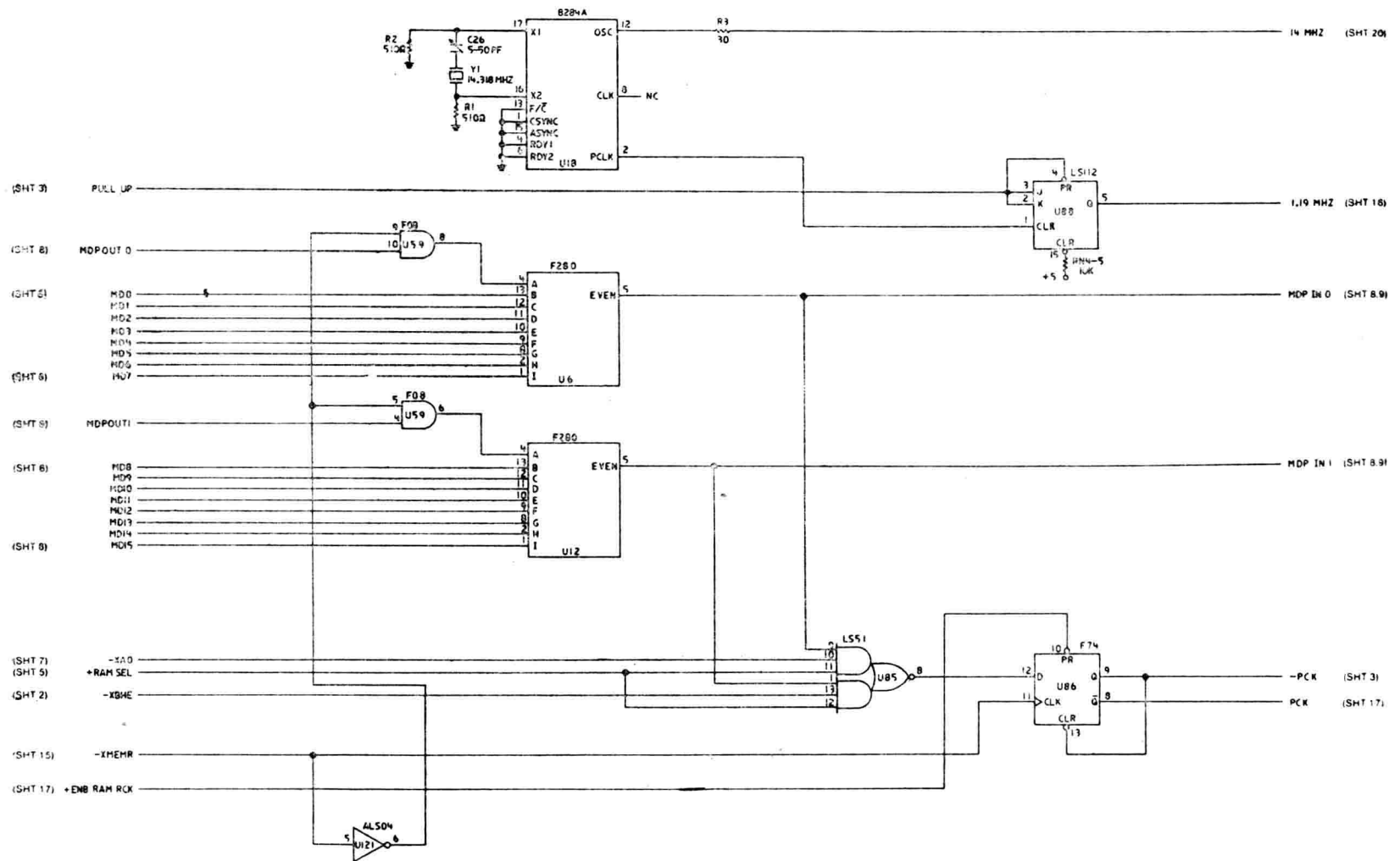
System Board (Sheet 11 of 22)
