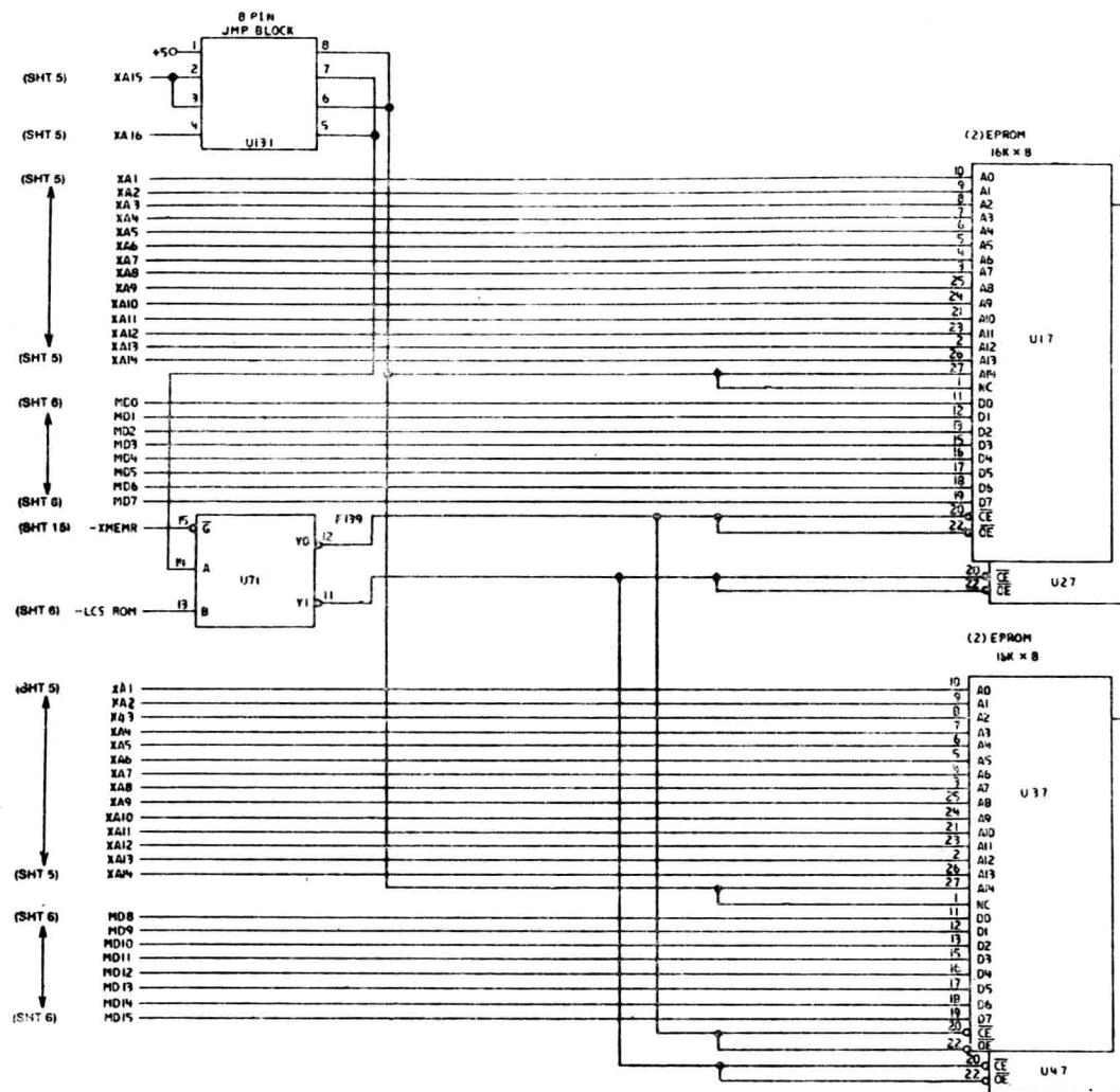
System Board (Sheet 10 of 22)
