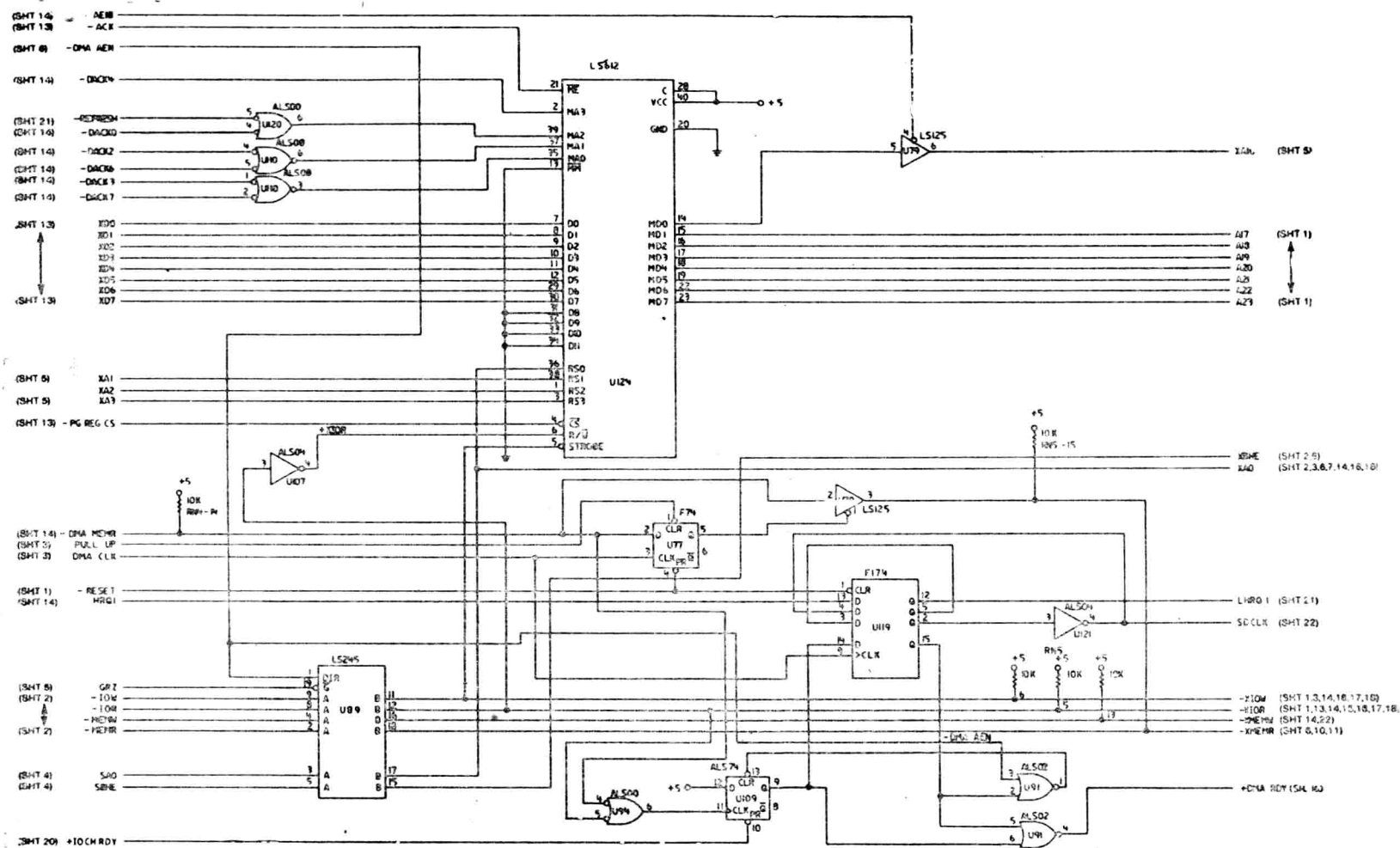
System Board (Sheet 15 of 22)
