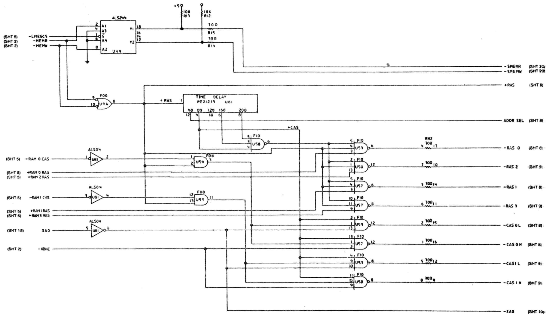
System Board (Sheet 7 of 22)
