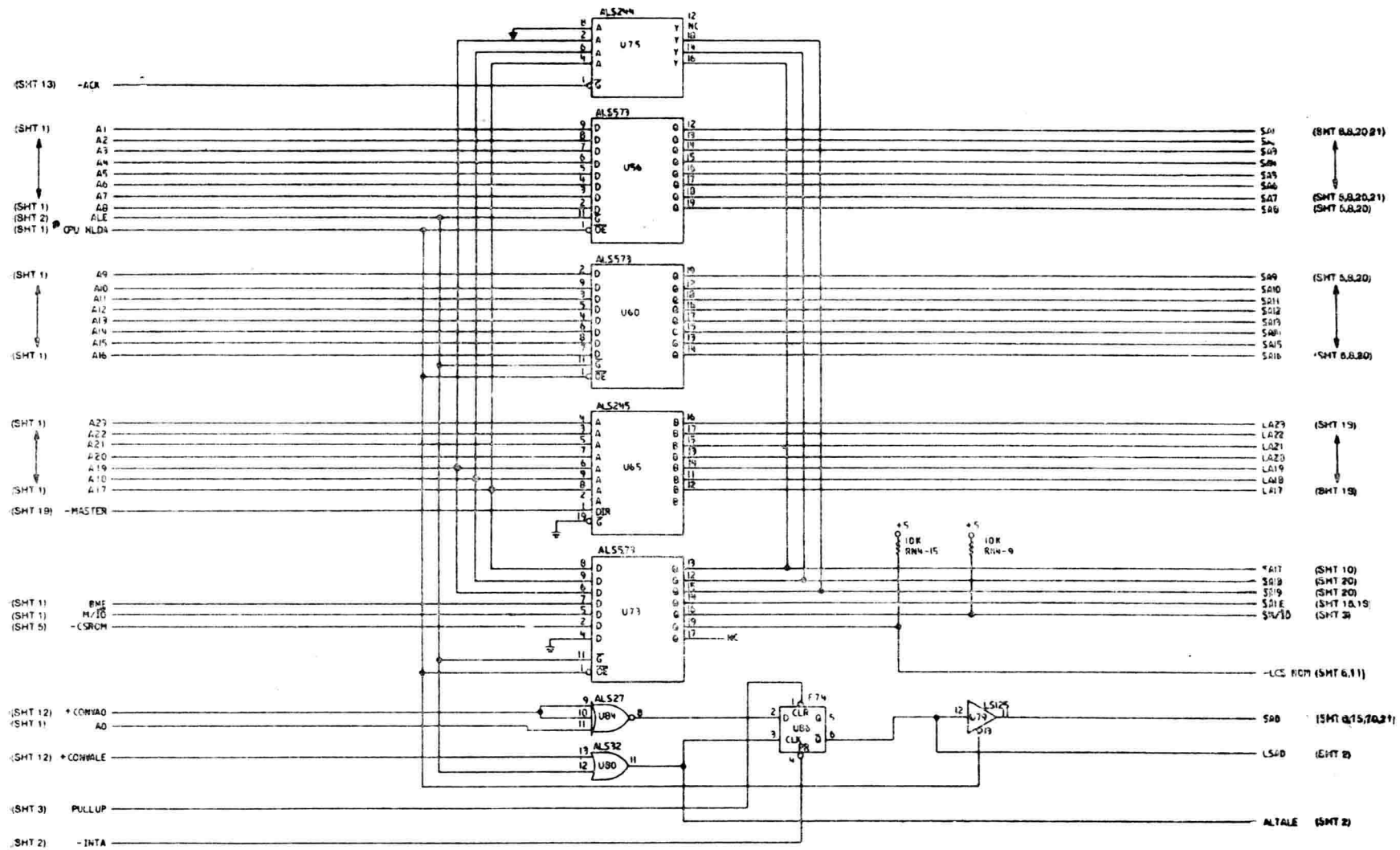
System Board (Sheet 4 of 22)
