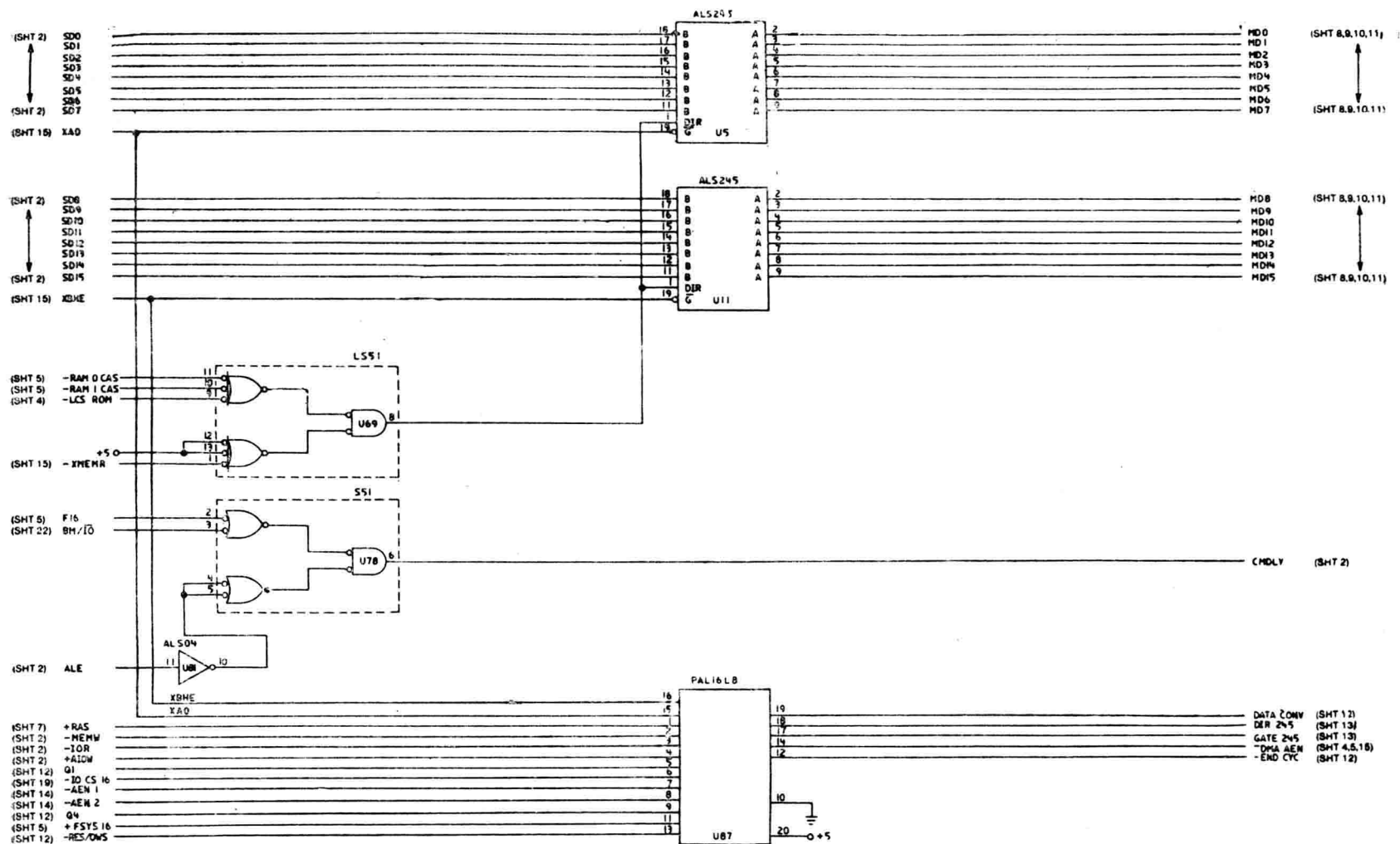
System Board (Sheet 6 of 22)
