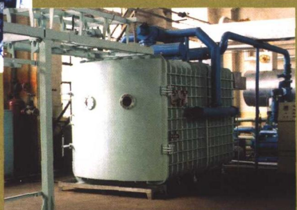
食品真空冷冻干燥设备 Food vacuum freezing drying equipment
