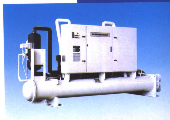
立式全封闭螺杆式冷水机组 Vertical Hermetic screw chillers
