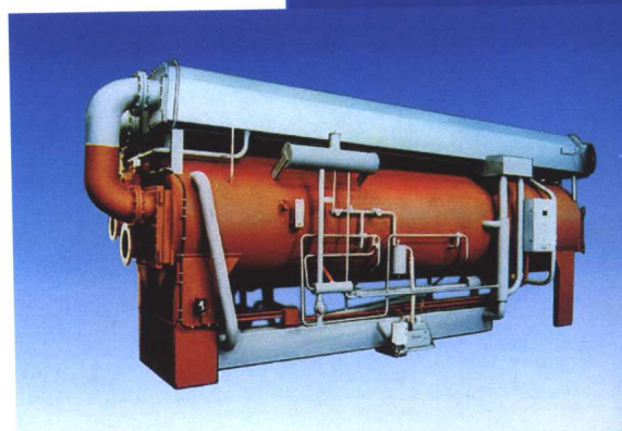
蒸汽型溴化锂吸收式冷水机 Steam Operated LiBr Absorption Water Chiller
