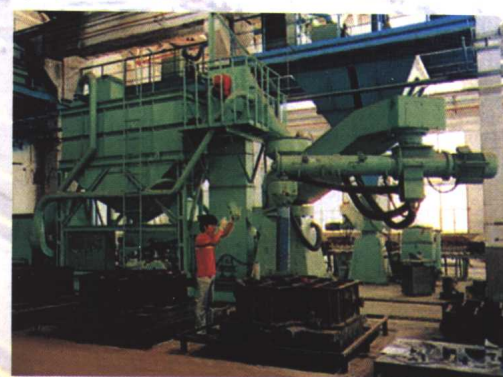
树脂砂铸造生产线 Resin Bonded Sand Casting Production Line
