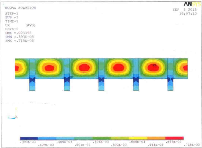
Figure 4: Displacement diagram under self-weight stress in X-direction.
