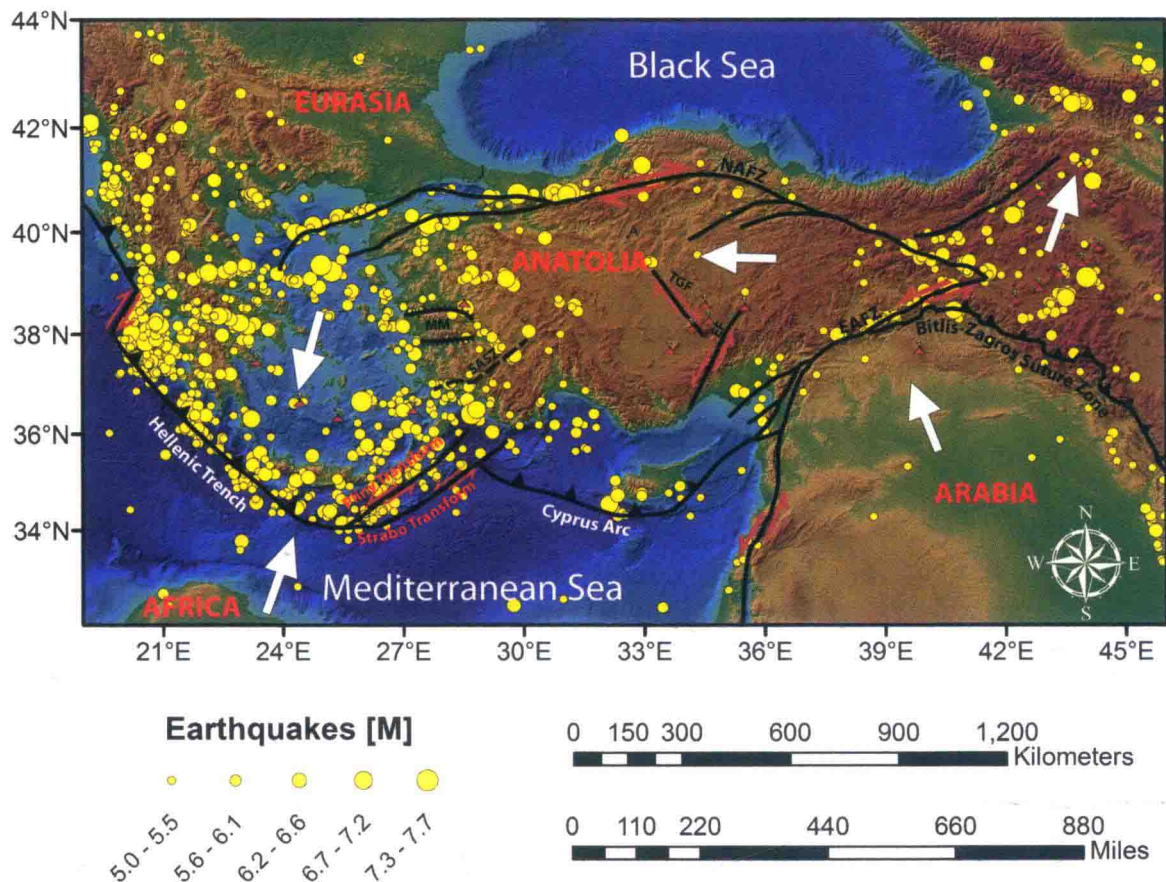
Figure 1.1 Digital elevation map of the eastern Mediterranean region showing major neotectonic structural features, volcanic centers (red triangles), and epicenters of the earthquakes ( M > 5.0 ) since 1950. A = Ankara; EAFZ = East Anatolian fault zone; EF = Ecemis fault; I = Istanbul; MM = Menderes Massif; NAFZ = North Anatolian fault zone; T = Thessaloniki; TGF = Tuz Golu fault.
