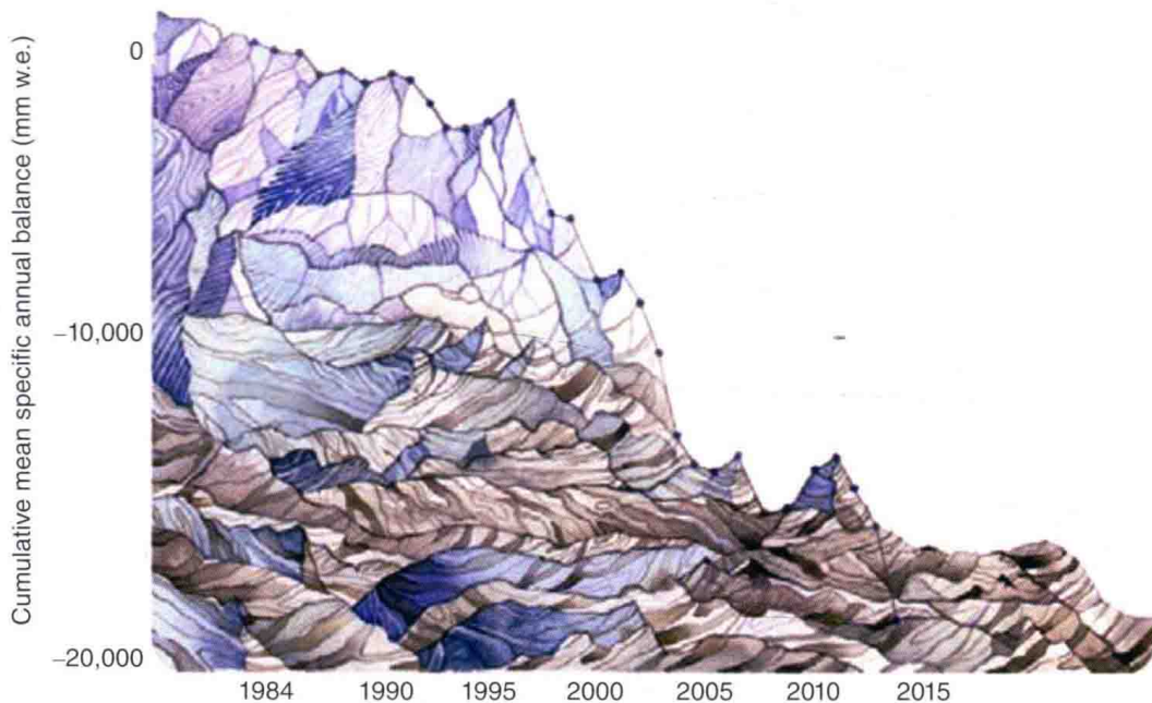
Figure 1 Decrease in glacier mass balance based on data from Peltó (2015a) to illustrate the dramatic decline in North Cascade glaciers, WA. (Watercolor, Jill Peltó 2015.)
