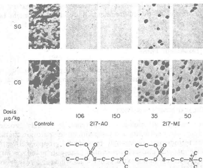
Fig. 5. The distribution of two organophosphates, a lipid-soluble tertiary base (217-AO) and a hydrophilic quaternary ammonium compound (217-MI) in the ganglion stellatum (SG) and ganglion ciliare (CG) of the cat. Note: the esterase activity (dark areas) is blocked intra- and extracellularly by the lipid-soluble compound and only in the extracellular space by the quaternary ammonium compound (McIsaac et al. , 59).
