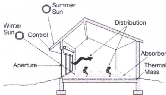
Elements of passive solar design, shown in a direct gain application
