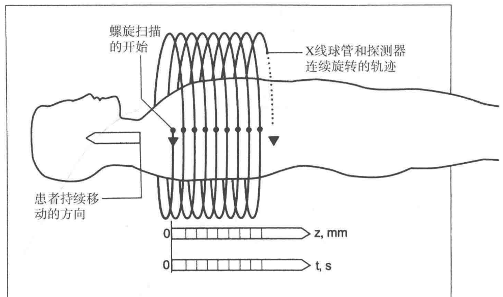
图 1-3 螺旋 CT 扫描原理。(From Kalender WA, Seissler W, Klotz E, Vock P: Spiral volumetric CT with single-breath-hold technique, continuous transport, and continuous scanner rotation. Radiology 176:181-183, 1990).
