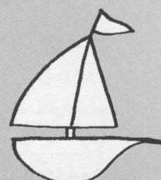
sailboat 帆船
