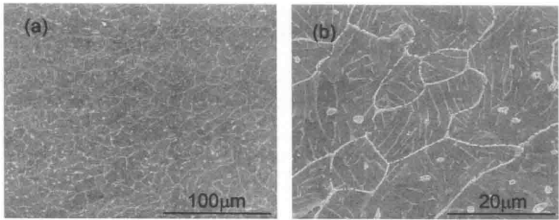
Figure 3. 5% TCP doped LENS™ processed Ti6Al4V composites under different magnifications. (a) Low magnification image and (b) high magnification image.
