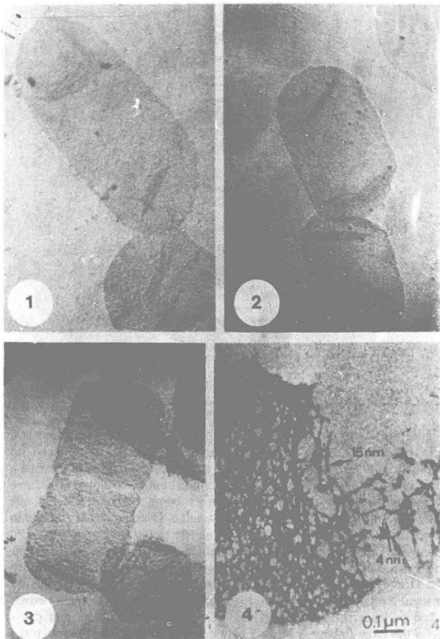
Figure 1.1: Electron Micrograph Showing Isolated Purified Sacculi from Escherichia coli . 1 and 2 show the purified sacculi which is in effect one enormous peptidoglycan molecule, 3 and 4 show the sacculi after treatment with specific endopeptidase. It can be seen that the glycan chains appear to run perpendicular to the long axis of the cell. Reproduced by permission, Verwer, R.W., Nanniga, N., Keck, W. and Schwartz, U. (1978) J. Bacteriol. , 136, 723.
