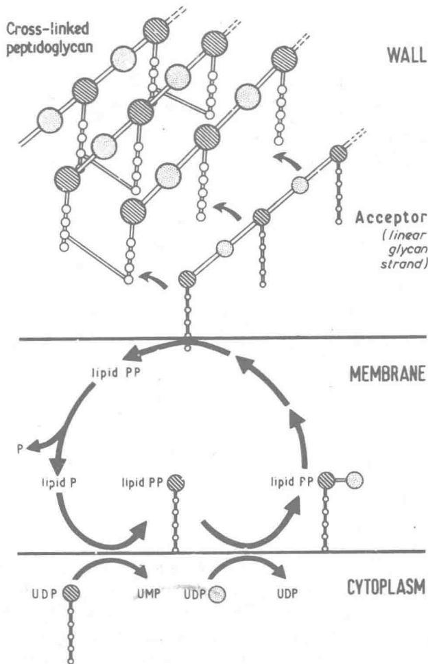
Figure 1.7: Sequence of Peptidoglycan Biosynthesis in Escherichia coli . Sugar nucleotides transfer N -acetylglucosamine (with its attached pentapeptide) and N -acetylmuramic acid to the C_{55} -isoprenoid lipid carrier which serves to translocate the precursor across the cytoplasmic membrane. At the outer face of the membrane the wall precursor is transferred to the growing linear glycan strand, releasing the isoprenoid for another round of synthesis. The acceptor glycan is subsequently cross-linked with existing wall peptidoglycan. (The symbols used for peptidoglycan structure are as in Figure 1.2)
