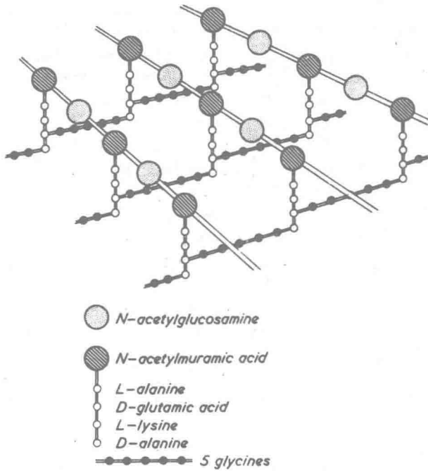
Figure 1.5: Structure of Peptidoglycan in Staphylococcus aureus
