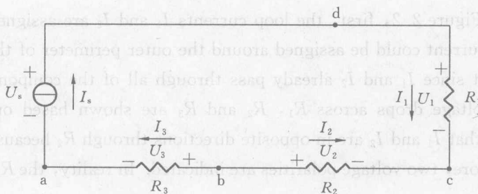
Figure 2.1 Circuit diagram
