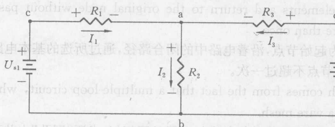
Figure 2.3 Example of circuit diagram for node voltage method
