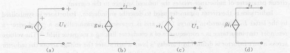
Figure 1.2 The circuit symbol for ideal dependent voltage sources
