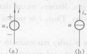
Figure 1.1 The circuit symbols
