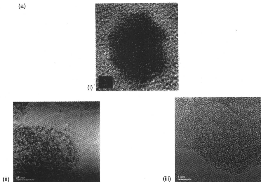
Figure 1.1 Classification of nanostructures. (a) Nanoparticles and nanopores (nanosized in three dimensions): (i) high-resolution TEM image of magnetic iron oxide nanoparticle, (ii) TEM image of ferritin nanoparticles in a liver biopsy specimen, and (iii) high-resolution TEM image of nanoporosity in an activated carbon. (b) Nanotubes and nanofilaments (nanosized in two dimensions): (i) TEM image of single-walled carbon nanotubes prepared by chemical vapour deposition, (ii) TEM image of ordered block copolymer film, and (iii) SEM image of silica nanotube formed via templating on a tartaric acid crystal. (c) Nanolayers and nanofilms (nanosized in one dimension): (i) TEM image of a ferroelectric thin film on an electrode, (ii) TEM image of cementite (carbide) layers in a carbon steel, and (iii) high-resolution TEM image of glassy grain boundary film in an alumina polycrystal. Images courtesy of Andy Brown, Zabeada Aslam, Sarah Pan, Manoch Naksata and John Harrington, IMR, Leeds
