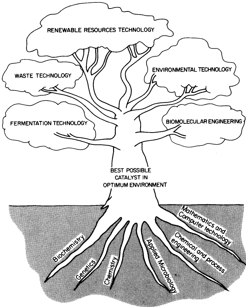
Fig. 1.2 Biotechnology tree.
