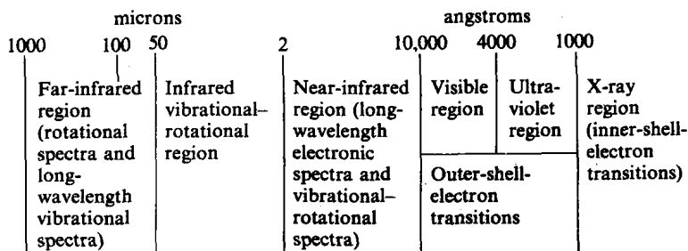
Figure 1-1. The electromagnetic spectrum.
