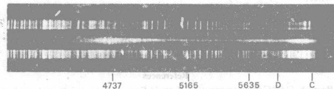
Spectrum of Halley's Comet, May 23, 1910. The bright-line spectrum shows the carbon bands, indicated by their wavelengths, and the D line of sodium, which lasted only a few days. In the spectrum of sunlight reflected by the comet's head, the dark Fraunhofer lines C and F are prominent. A comparison spectrum appears above and below. (Lowell Observatory photograph)
