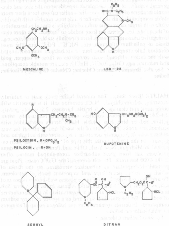
Structures of some hallucinogenic drugs.
