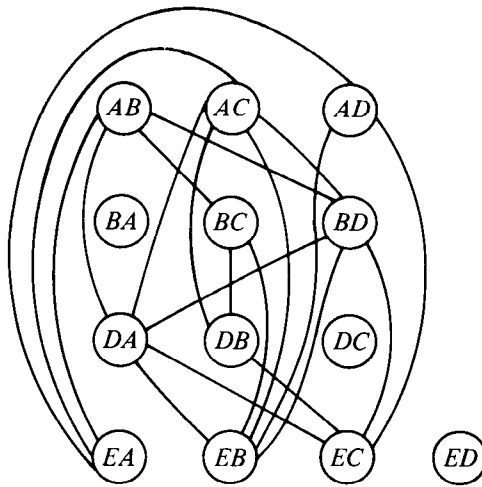
Fig. 1.2. Graph showing incompatible turns.
