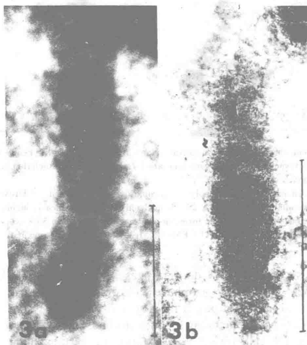
FIG. 3. Chromosome of Dinoflagellate ( Cryptothecodinium cohnii ). One micron section. (a) Photographed at 80 kV with Siemens Elmiskop 1. (b) photographed at 1000 kV, with 1.5 MeV microscope in Toulouse, France. The 2 nm thick DNA filaments in this chromosome are resolved in the high voltage electron microscope, but not in the conventional electron microscope.
