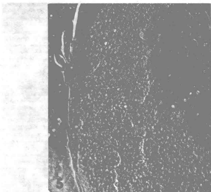
FIG. 5. Freeze-etching of nucleus in spleen of salamander. The chromatin shows cross fractures through the 20nm native fibers (arrows).
