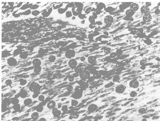
Figure 6: A deformed dolomite–calcite marble from Sardinia containing spherical fossil objects (oolites) about three millimetres in size. Oolites made of dolomite (black circles) are not deformed. Oolites made of calcite (gray), a weaker solid, are smeared out in S forms.
