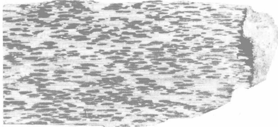
Figure 3: Cross-sectional view of a spotted phyllite from Cornwall, showing the intense stretching of spots (chlorite) in the quartz-rich (white) matrix.
