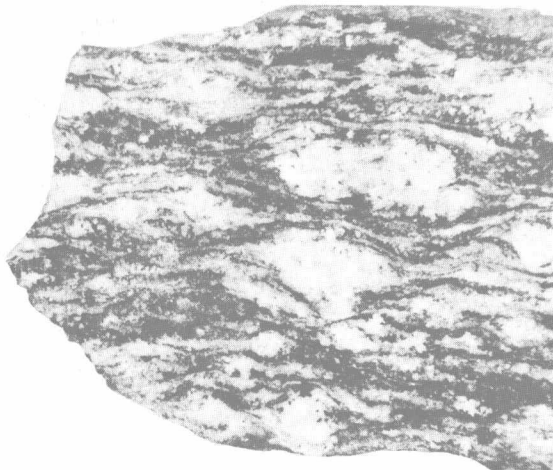
Figure 4: Typical granitic gneiss from Africa with large crystals of feldspar and a matrix containing dark biotite flowing around them.
