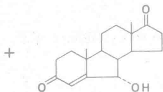
6 \alpha -Hydroxy-B-norandrost-4-ene-3, 17-dione (35.6%)
