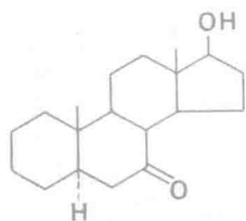
17 \beta -Hydroxy-5 \alpha -androstan-7-one
