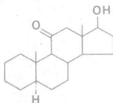
17 \beta -Hydroxy-5 \alpha -androstan-11-one (28%)
