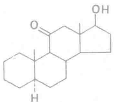
17 \beta -Hydroxy-5 \alpha -androstan-11-one
