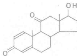
17β-Hydroxyandrosta-1, 4-diene-3, 11-dione (6%)
