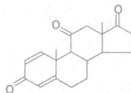
Androsta-1, 4-diene-3, 11, 17-trione (2%)
