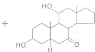
3β, 11α-Dihydroxy-5α-androstan-7-one (5%)
