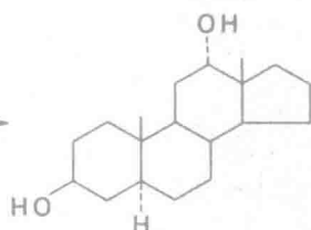
3β, 12α-Dihydroxy-5α-androstane (10%)
