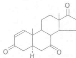
5 \alpha -Androst-1-ene-3, 7, 17-trione
