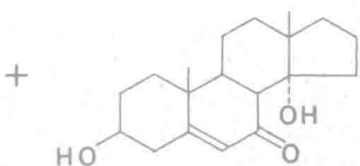
3β, 14α-Dihydroxyandrost-5-en-7-one (19%)
