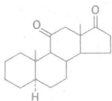
5 \alpha -Androstane-11, 17-dione
