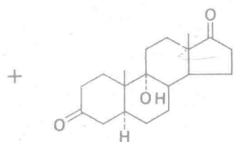
9α-Hydroxy-5α-androstane-3, 17-dione (2%)
