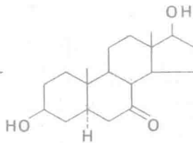
3 \beta , 17 \beta -Dihydroxy-5 \alpha -androstan-7-one (24%)
