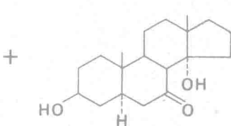
3β, 14α-Dihydroxy-5α-androstan-7-one (9%)
