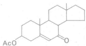
3β-Acetoxyandrost-5-en-7-one
