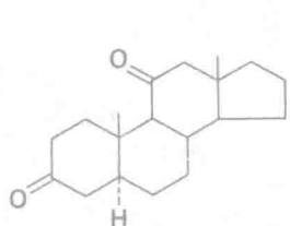
5α-Androstane-3, 11-dione
