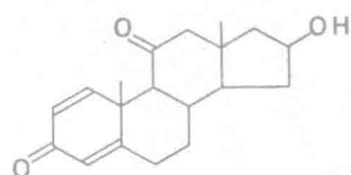
16β-Hydroxyandrosta-1, 4-diene-3, 11-dione (4%)
