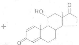
11 \alpha -Hydroxyandrosta-1, 4-diene-3, 17-dione (16%)
