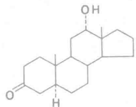
12α-Hydroxy-5α-androstan-3-one
