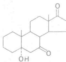
5 \alpha -Hydroxy-5 \alpha -androstane-7, 17-dione (6%)
