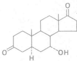
7α-Hydroxy-5α-androstane-3, 17-dione (10%)
