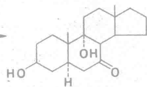
3β, 9α-Dihydroxy-5α-androstan-7-one (23%)
