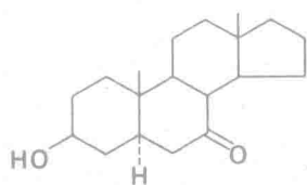
3β-Hydroxy-5α-androstan-7-one
