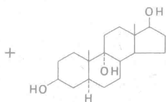
3β, 9α, 17β-Trihydroxy-5α-androstane (8%)
