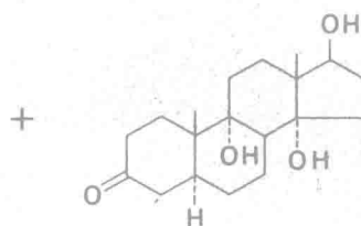
9α, 14α, 17β-Trihydroxy-5α-androstan-3-one (2%)
