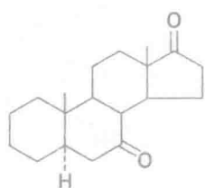
5 \alpha -Androstane-7, 17-dione
