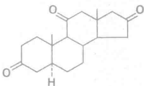
5α-Androstane-3, 11, 16-trione (2%)
