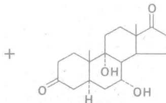
7α, 9α-Dihydroxy-5α-androstane-3, 17-dione (7%)
