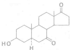
3 \beta -Hydroxy-5 \alpha -androstane-7, 17-dione (6%)
