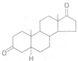
5α-Androstane-3, 17-dione
