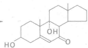
3β, 9α-Dihydroxyandrost-5-en-7-one (21%)
