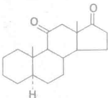
5 \alpha -Androstane-11, 17-dione (25%)
