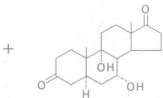
7 \alpha , 9 \alpha -Dihydroxy-5 \alpha -androstane-3, 17-dione (13%)
