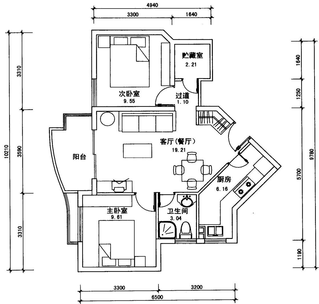
H4型户型平面图
