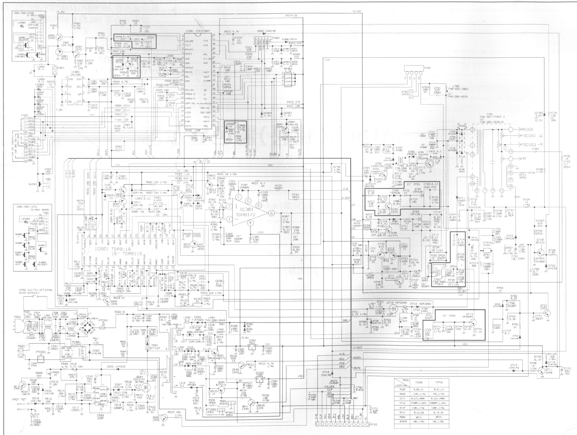
AOpen A50P/A70P 彩色显示器电路原理图(1/2)
