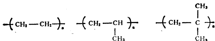
聚乙烯
