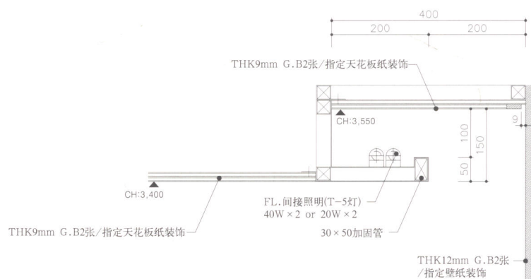
饭厅天花板细部/ceiling detail(dining room)
