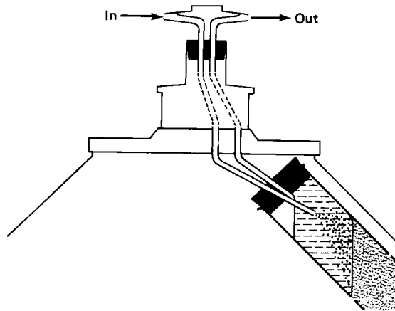
Figure 1.1. Simplified diagram of the continuous-flow adaptor for Sorvall SS-34 centrifuge rotor. Liquid can be passed through at several hundred milliliters per minute, collecting particulate matter up to 300 cm 3 in volume.
