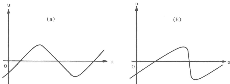
Fig. 4. Sketch of the nonlinear steepening of a wave as it develops. (a) t = 0 . (b) Later.
