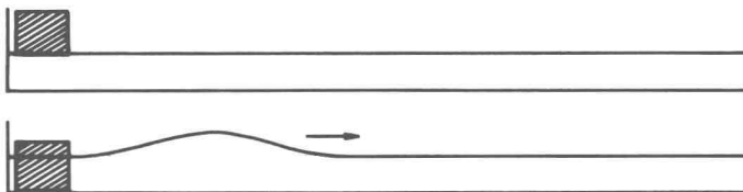
Fig. 2. The configuration and parameters for description of a solitary wave.
