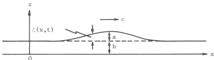
Fig. 2. The configuration and parameters for description of a solitary wave.
