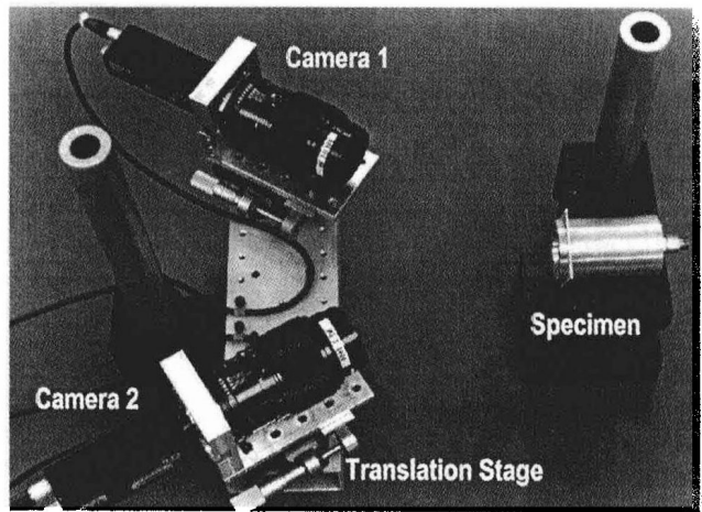
Figure 3: Typical system for three-dimensional displacement measurements.
