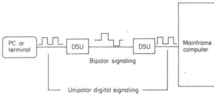
Figure 2.3 Transmitting Data on a Digital Network
