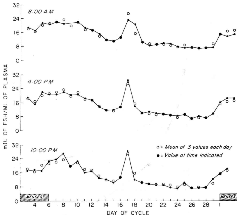
FIG. 4. Plasma FSH concentrations measured in samples taken at 8:00 AM (upper), 4:00 PM (middle), and 10:00 PM (lower) daily during a complete menstrual cycle (●—●). Means of concentrations in all three samples, (○) are shown for comparison.
