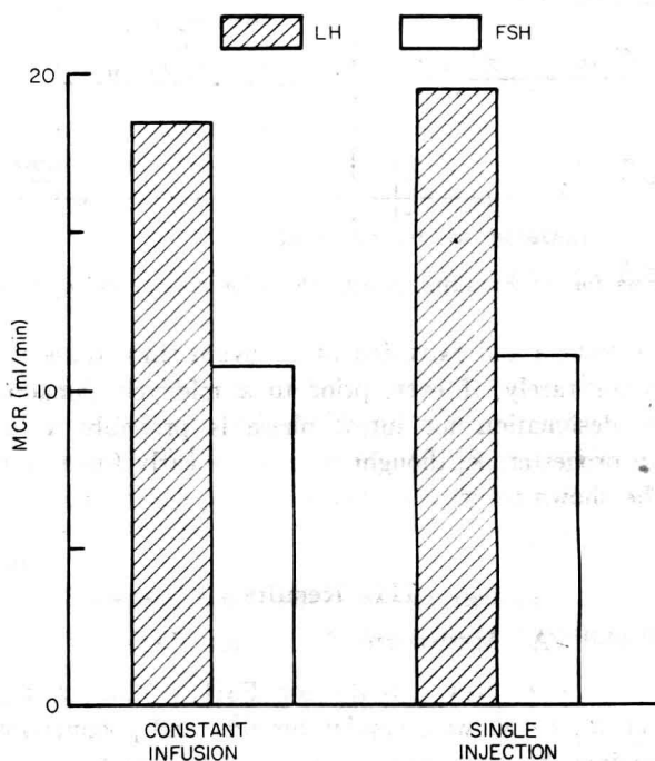
FIG. 2. Average metabolic clearance rates (MCR) for FSH and LH determined by a method based upon continuous infusion and by a method based upon a single injection of isotopically labeled hormone.
