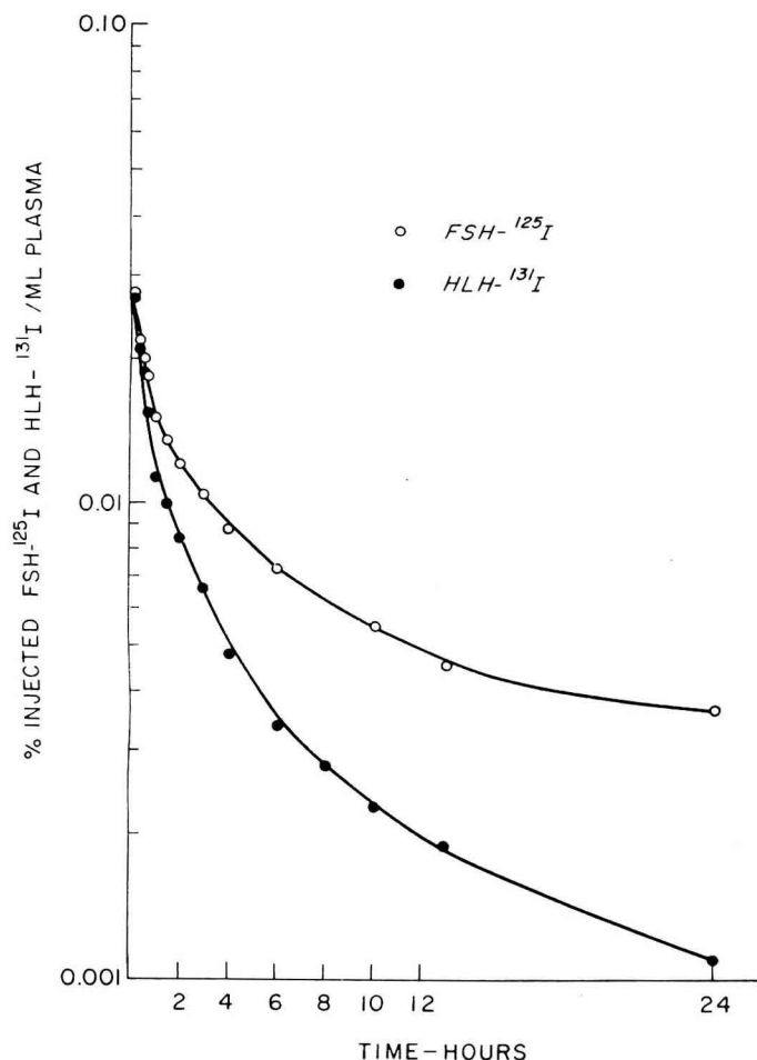
FIG. 3. Percent of injected dose of FSH- 125 I and LH- 131 I remaining in plasma at varying times following simultaneous injection of the two preparations in the same subject. Reprinted from Coble et al. (1969).
