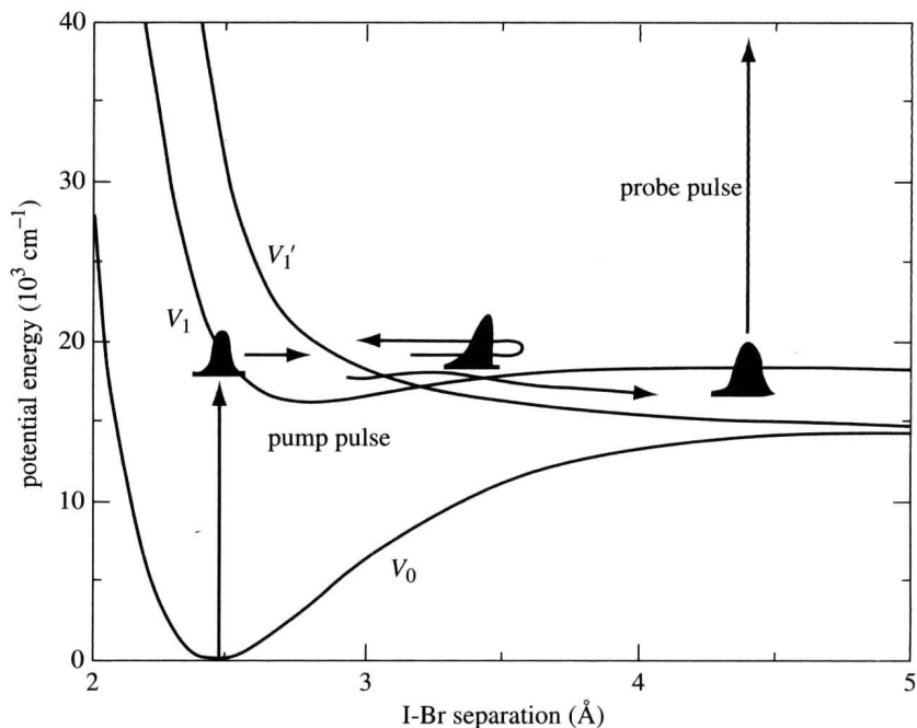
Figure 1.3. Real-time femtosecond spectroscopy of molecules can be described in terms of optical transitions excited by ultrafast laser pulses between potential energy curves which indicate how different energy states of a molecule vary with interatomic distances. The example shown here is for the dissociation of iodine bromide (IBr). An initial pump laser excites a vertical transition from the potential curve of the lowest (ground) electronic state V_0 to an excited state V_1 . The fragmentation of IBr to form \text{I} + \text{Br} is described by quantum theory in terms of a wavepacket which either oscillates between the extremes of V_1 or crosses over onto the steeply repulsive potential V_1' leading to dissociation, as indicated by the two arrows. These motions are monitored in the time domain by simultaneous absorption of two probe-pulse photons which, in this case, ionise the dissociating molecule.
